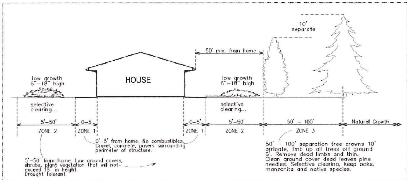
FIGURE 4907.2 MEASUREMENTS OF FUEL MODIFICATION DISTANCE
